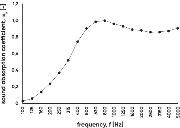
Absorption of Treehouse external panels
