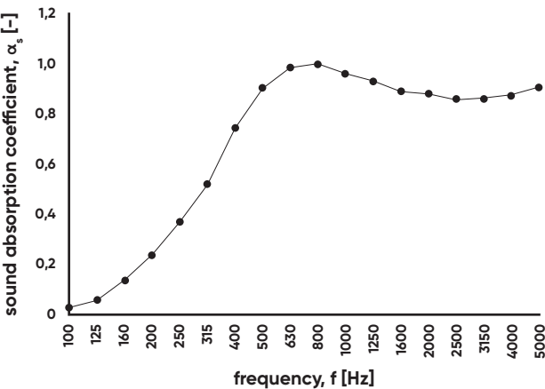
absorption of Treehouse external panels
